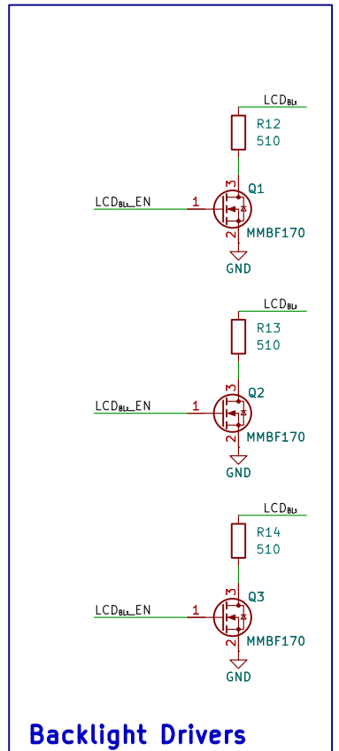
LCDs
